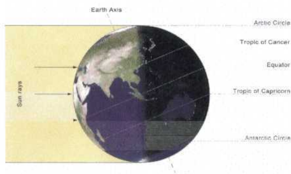
on the day of Northern solstice
