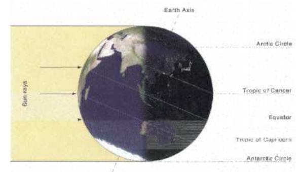
on the day of Southern solstice
