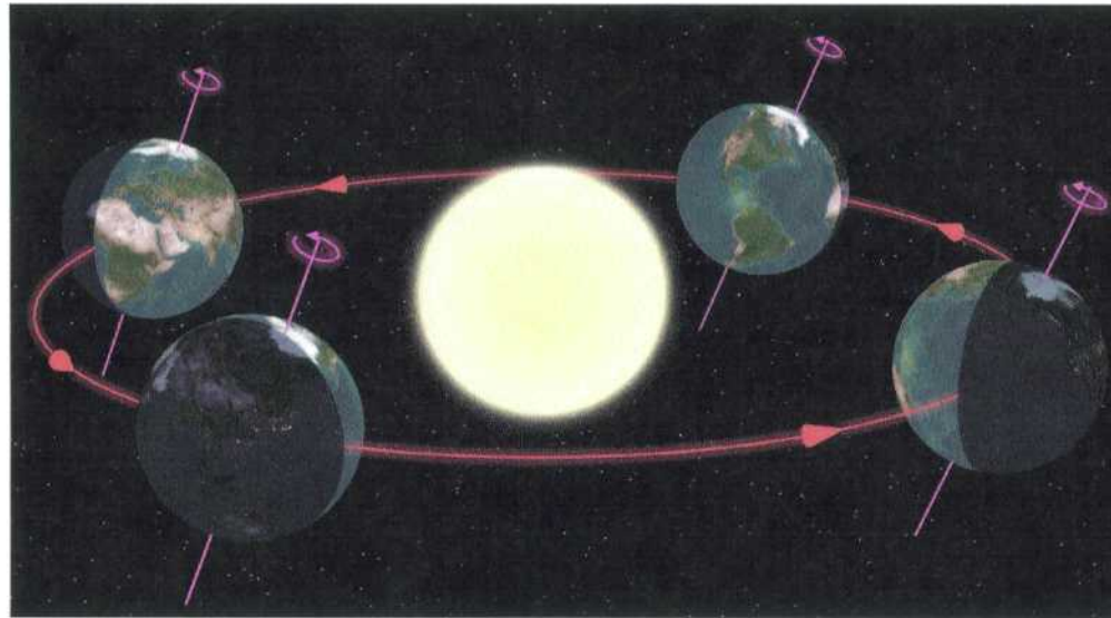
Far right: December solstice
