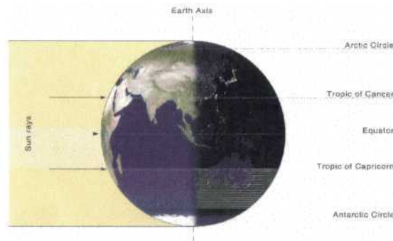
on the day of Equinox
